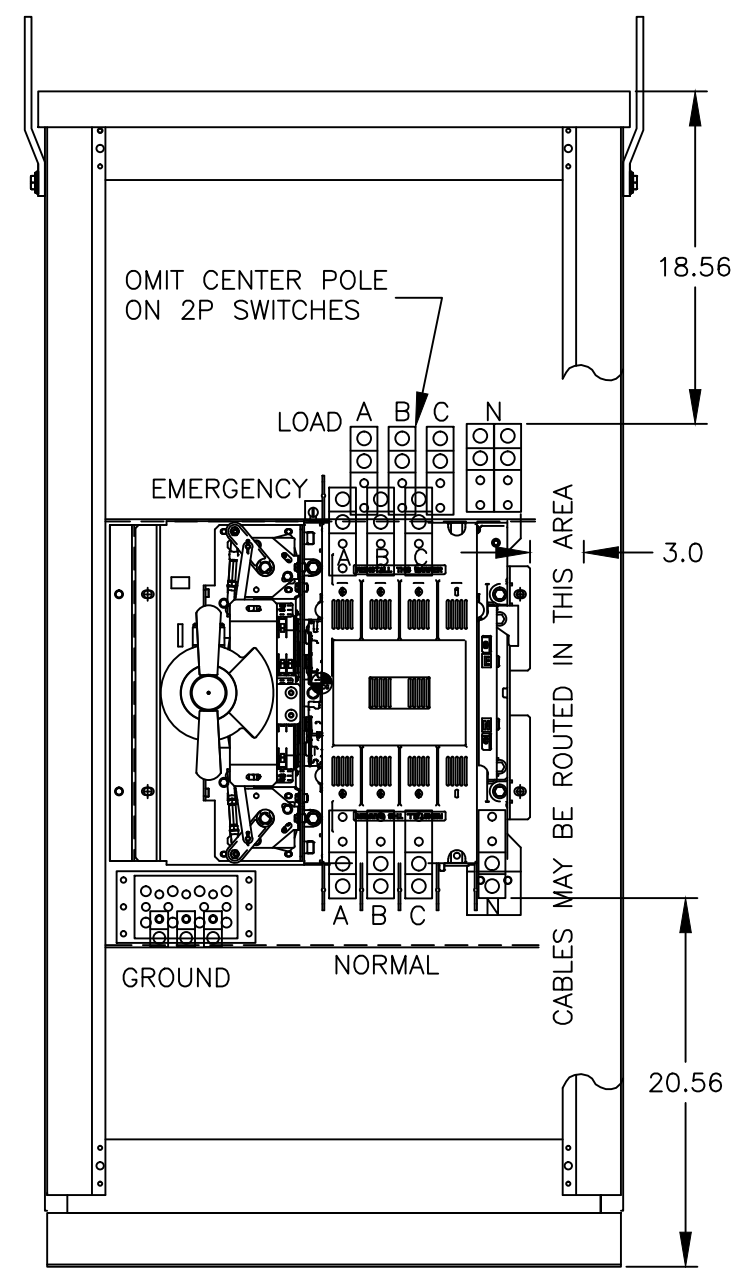
"FRONT VIEW" "WITHOUT COVER"
