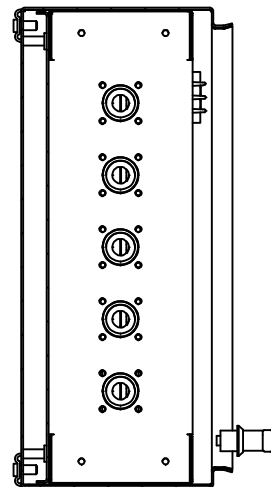
SECTION B-B Input Cam Placement
