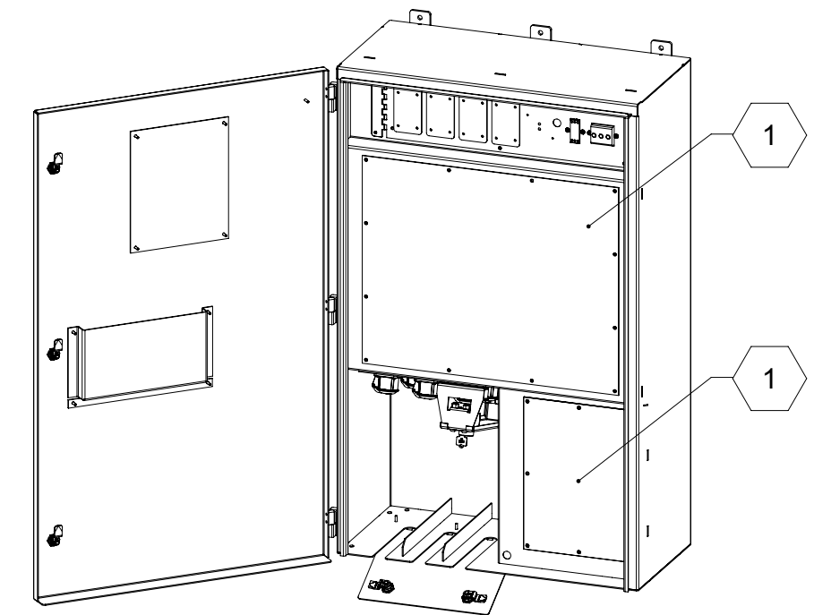
DIMETRIC VIEW OPEN 1:16 SCALE
