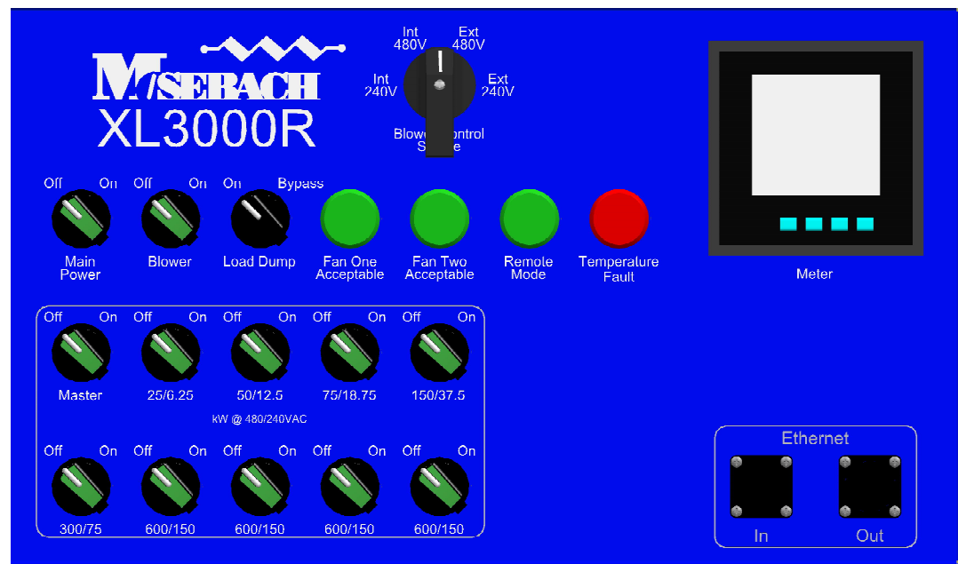
Control Detail
