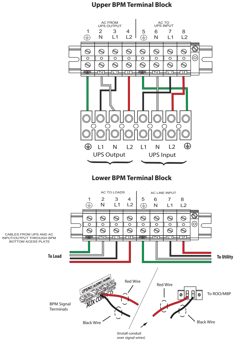
Figure 13. 9PX Split Phase UPS to BPM Connection Diagram with Signal Inputs
