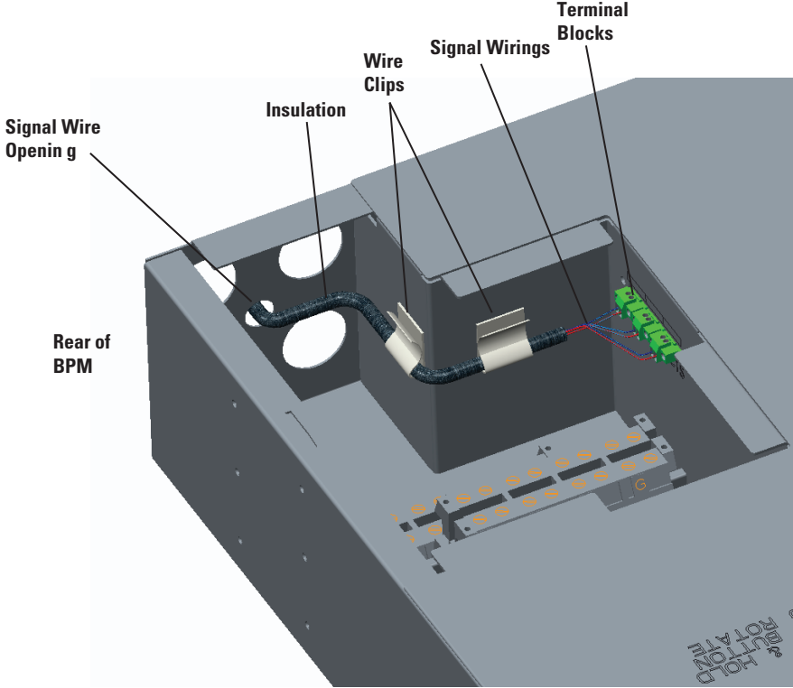
Figure 10. Signal Wire Routing
