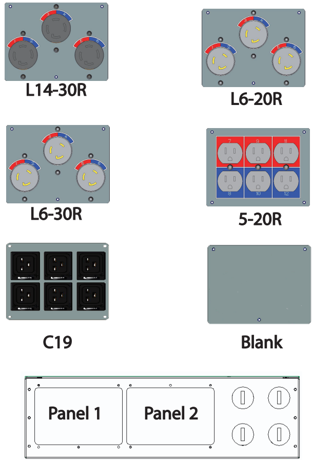
Figure 20. Rear Panel Outlet Options
