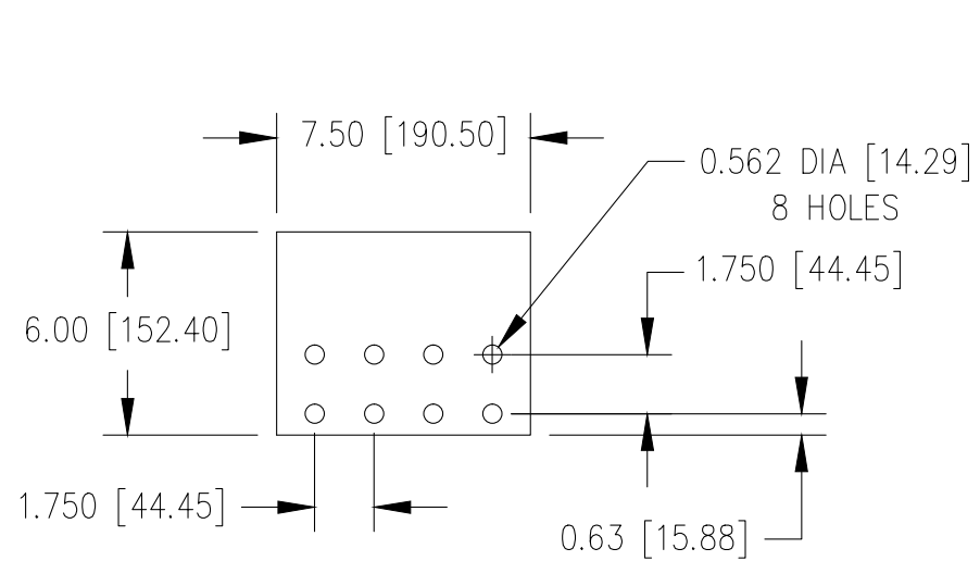
LOAD CONNECTION BUS BAR DETAIL BUS BARS ARE 0.25 [6.35] THICK TIN PLATED COPPER TYPICAL FOR ALL THREE PHASES (SCALE: NONE)
