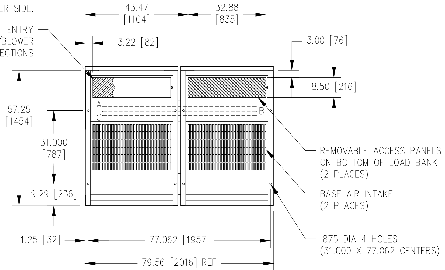
VIEW A—A
