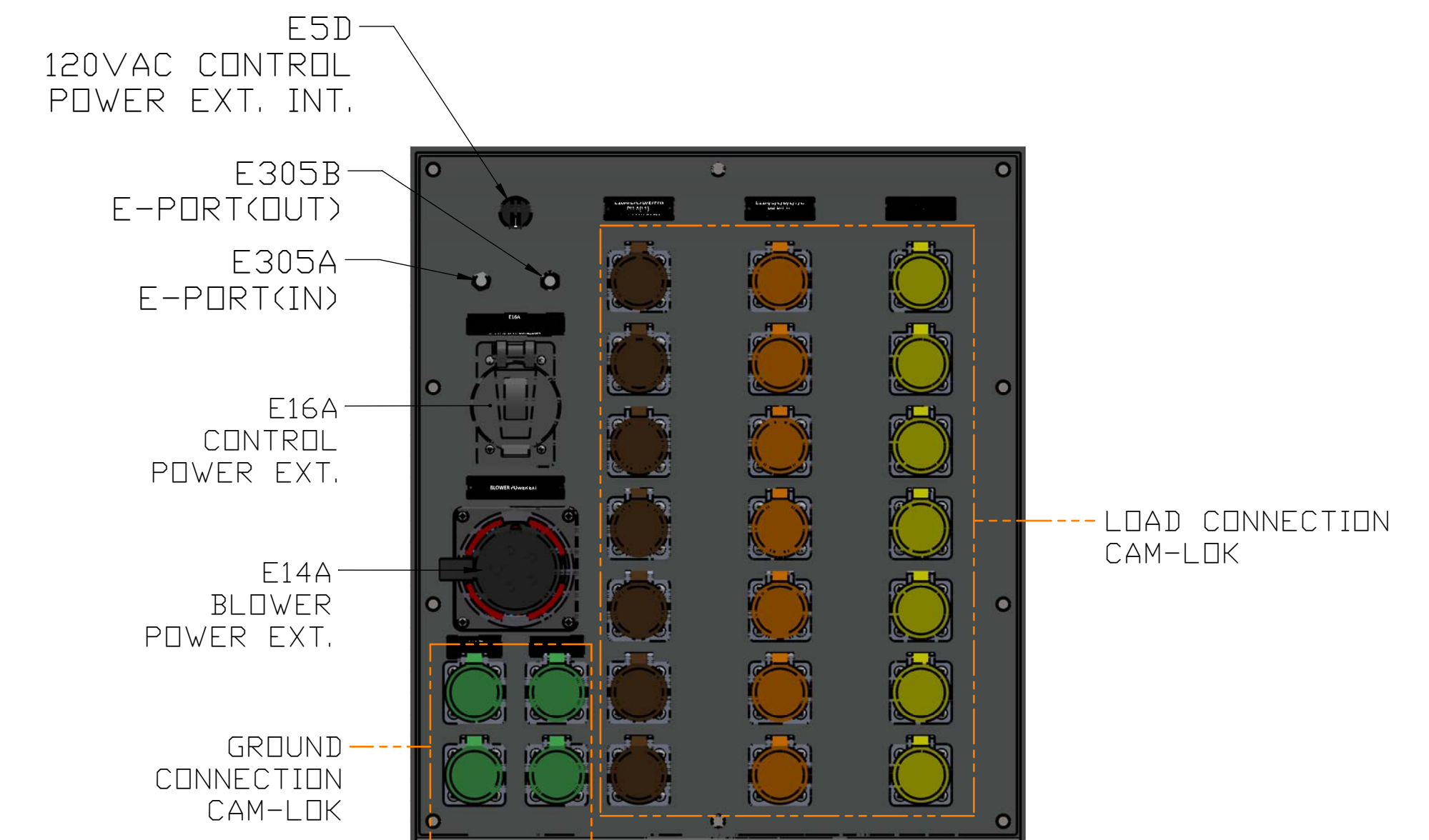
DETAIL B
