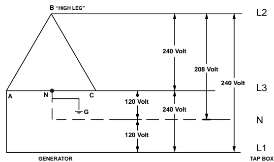
Delta 4-Wire Connection [Delta 3-Wire eliminates Neutral (N) connection (dashed line)]
