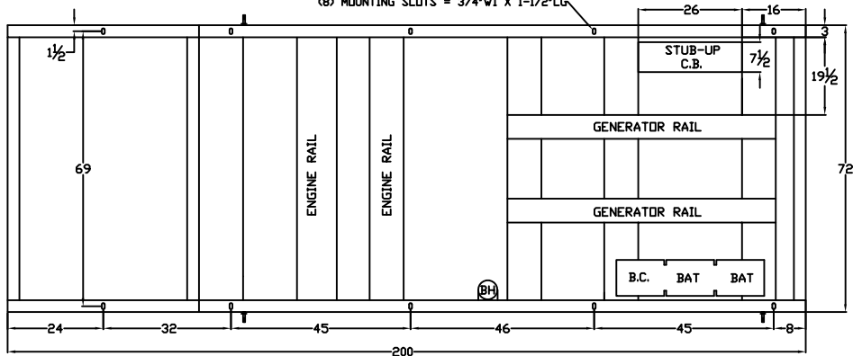
FRAME VIEW
