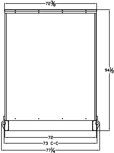
RADIATOR END VIEW
