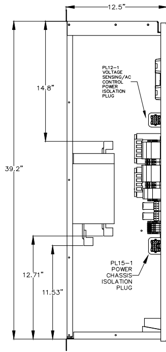
LHS VIEW (SIDE COVER REMOVED)
